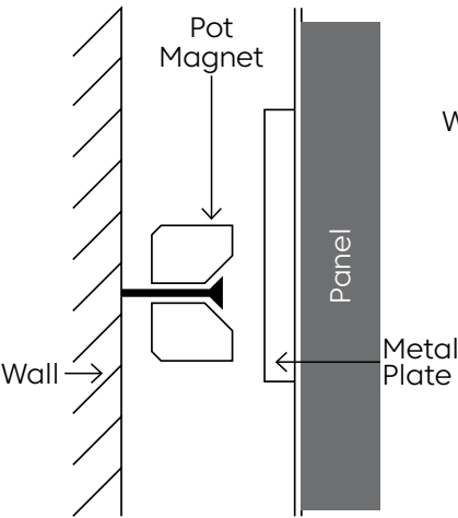
Wall Pot Magnet Install Metal Plate
