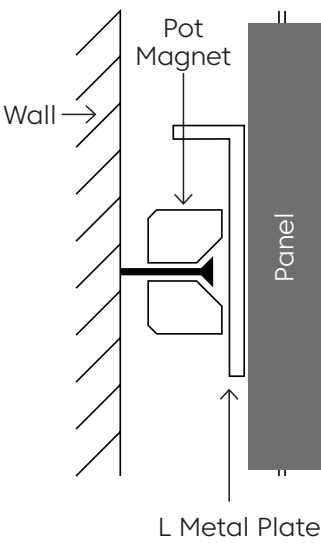
Wall Pot Magnet Install L Plate + Metal Plate
