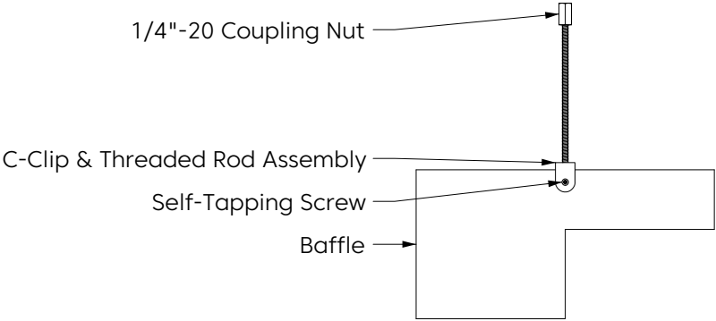
Threaded Rod
