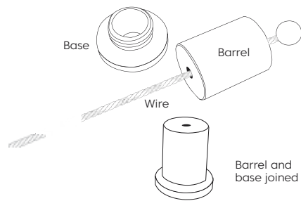
Cable gripper
