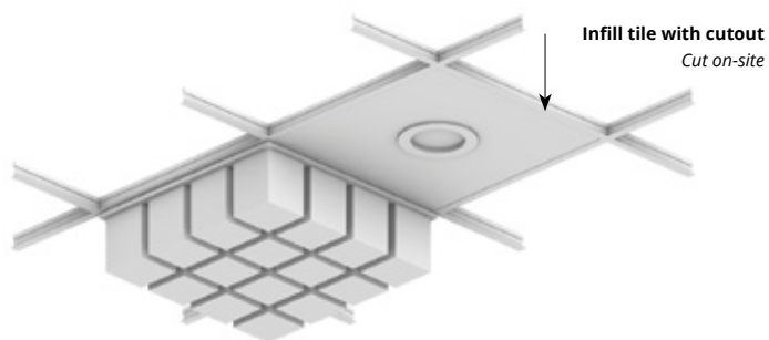
Recessed light
